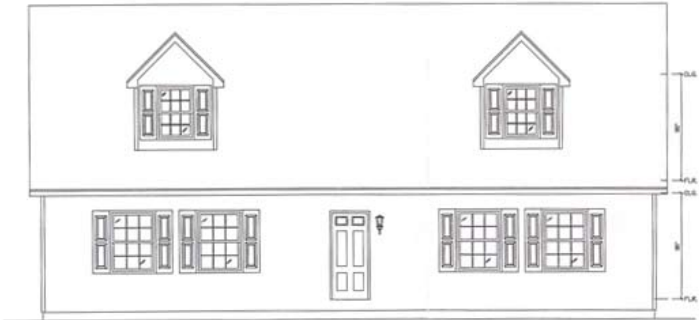
FRONT ELEVATION
