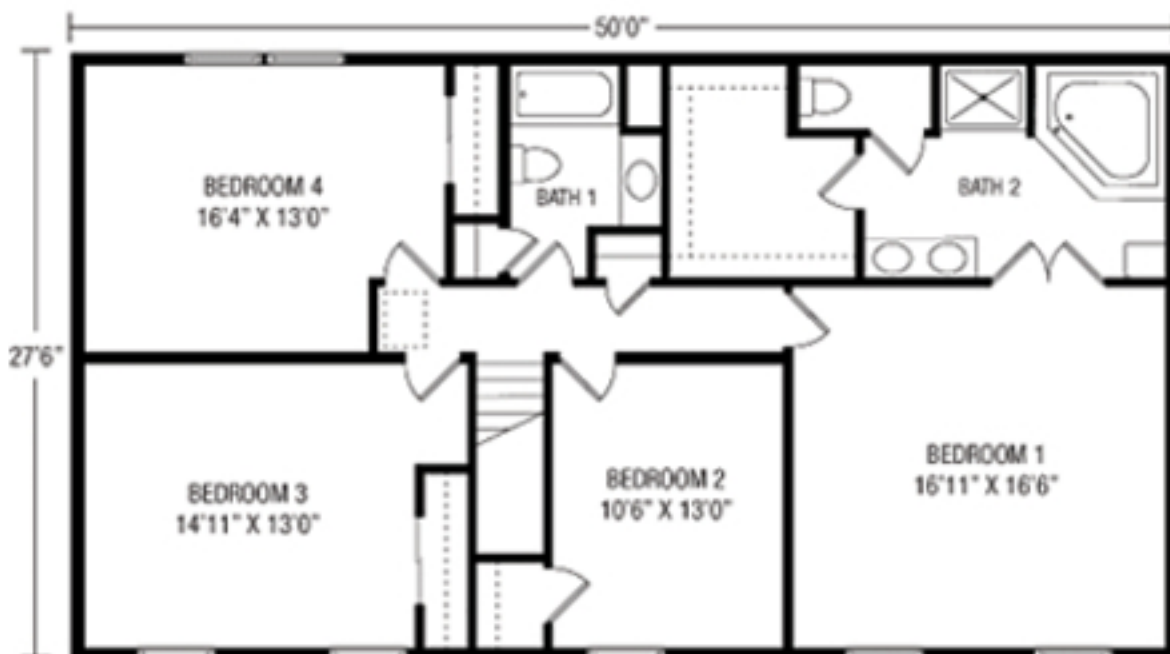
second floor
